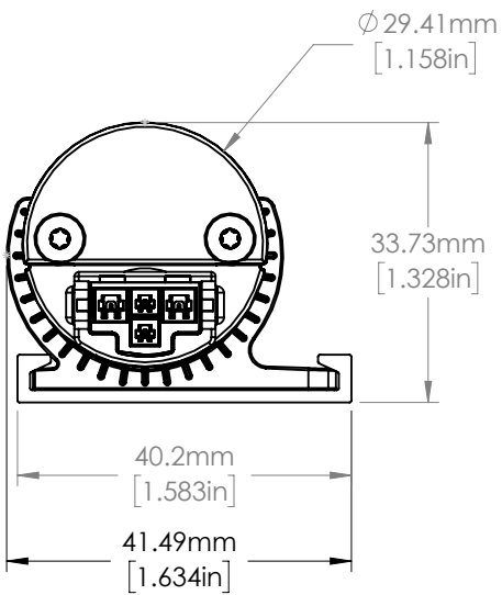
Fixture w/ track
