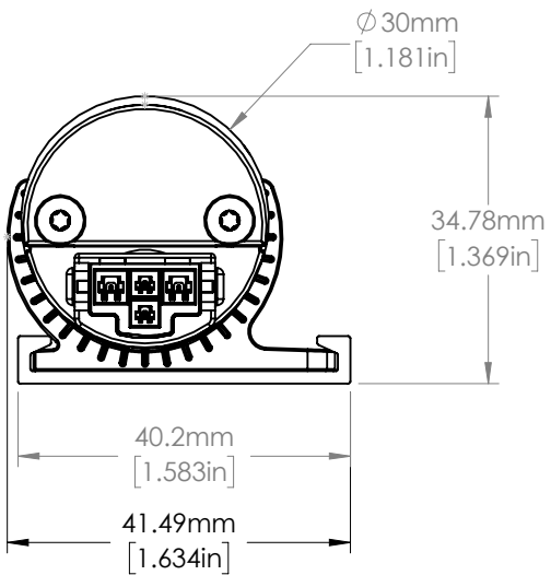
Fixture w/ track and frosted lens
