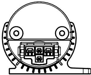
Fixture w/ track and frosted lens
